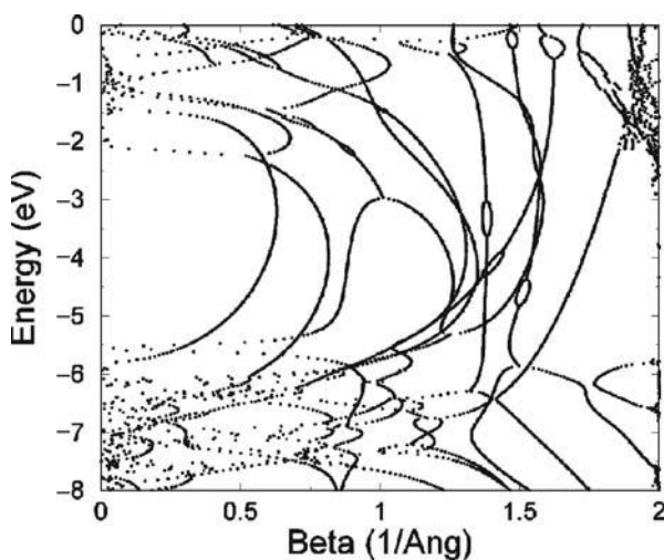
Fig. 7.5 The complex band structure of m- \text{HfO}_2 in the near gap region. The charge neutrality level is 2.3 eV above the band valence band top as calculated. The band gap is calculated to be 3.5 eV, therefore the rescaled value of the charge neutrality level is estimated to be 3.8 eV
