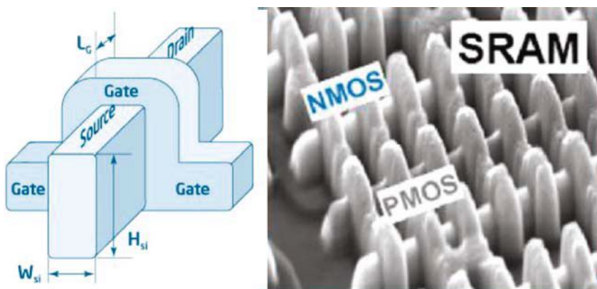
Fig. 6.3 Non-classical device structures. Left : a schematic of a FinFET; right : an SEM photo of multileg NMOS and PMOS FinFET structures forming part of an SRAM. Reprinted with permission from R. Chau
