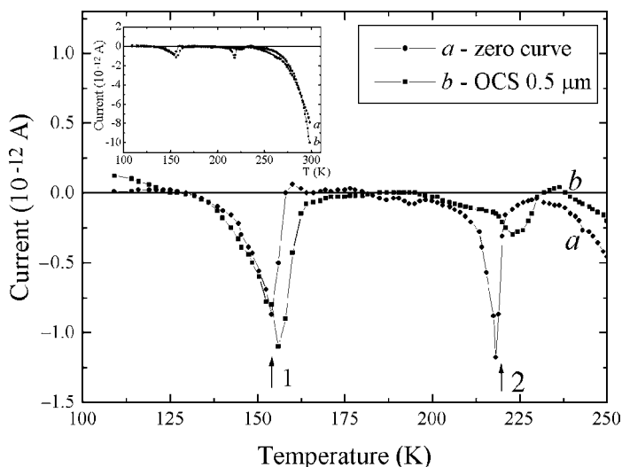
Fig. 8.14 OCS discharge current in MQW structure: ( a ) zero (no illumination) curve; ( b ) OCS ( \lambda = 0.5 \mu\text{m} ) curve [8]. Reprinted from Solid State Electronics, M. L. Ciurea, V. Iancu, and R. M. Mitroi, "Trapping Phenomena in Silicon-Based Nanocrystalline Semiconductors", 51 , 1328–1337, 2007, Copyright © 2007, with permission from Elsevier
