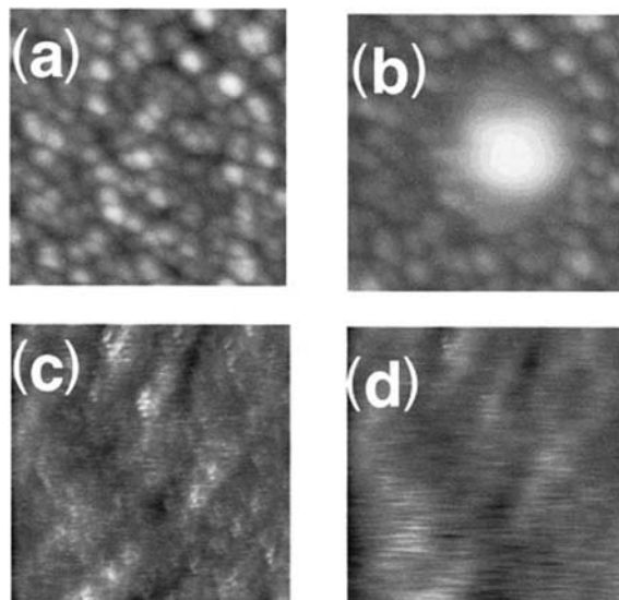
Fig. 8.11 AFM image of a SiO 2 film containing Si nanocrystals made by Si + ion implantation and annealing: (a) before charging and (b) after charge transfer [30]. Lateral size of the images is 5 \mu\text{m} : black to white (vertical) scale is 15 nm for (a) and 25 nm for (b). Similar images for Ar + ions' implantation: (c) before charging and (d) after charge transfer [30]. Lateral size for both images is 1 \mu\text{m} : black to white (vertical) scale is 1.5 nm. Reused with permission from E. A. Boer, M. L. Brongersma, H. A. Atwater, R. C. Flagan, and L. D. Bell, Applied Physics Letters , 79 , 791, 2001. Copyright © 2001, American Institute of Physics
