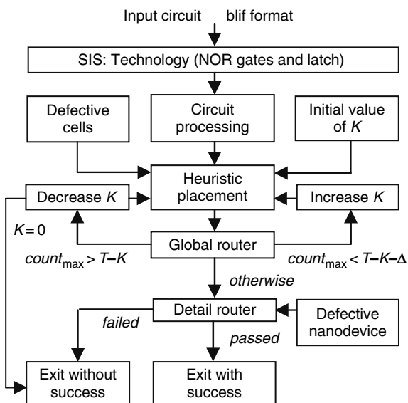
Fig. 4.18 CMOL FPGA design flow used in this work
