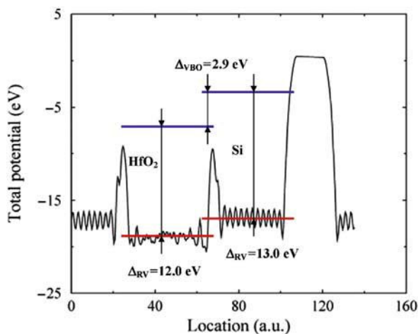
Fig. 7.4 The valence band offset between Si and \text{HfO}_2 is calculated using the reference potential method. The average reference potential is indicated with red lines , and the valence band maxima with blue lines . The discontinuity is estimated to be 2.9 eV (See Color Insert)
