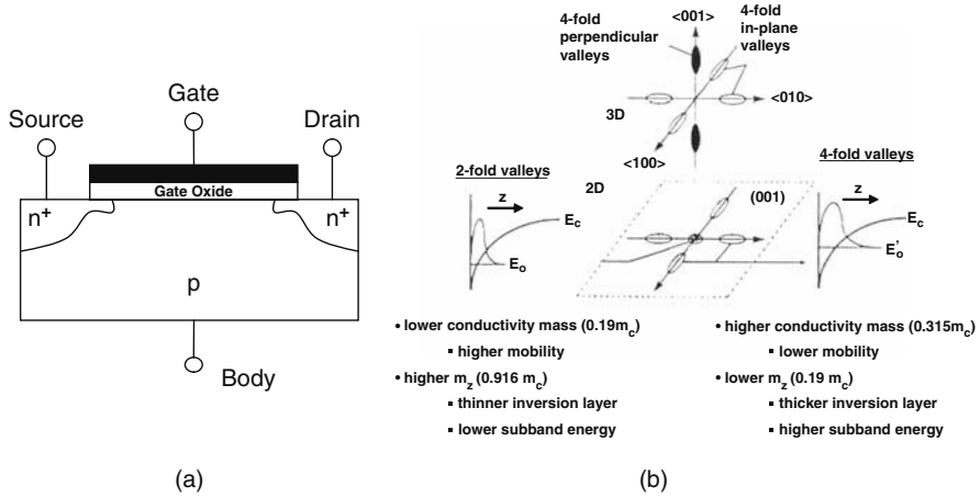
Fig. 6.11 Quasi-2D system formed at the Si/SiO 2 interface in a MOSET (metal oxide semiconductor field effect transistor) device. (a) Cross-section of the device. (b) Effect of the multi-valley conduction band structure on quantization for [100] Si (with permission from D. Vasileska, private communication)
