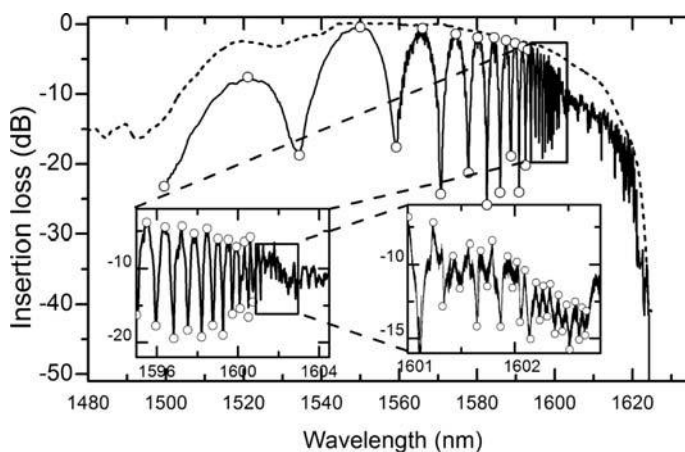
Fig. 11.22 The transmission spectra of a photonic crystal waveguide ( dashed ) and a photonic crystal Mach–Zehnder interferometer ( line ) with two slightly asymmetric arms. Insets show the fine details of the MZI spectrum (courtesy of Yurii A. Vlasov)
