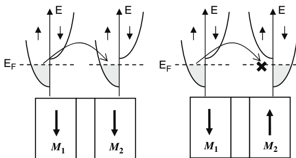
Fig. 5.8 Schematic picture of tunneling magnetoresistance
