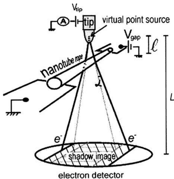
Fig. 8.18 LEEPS microscope set-up [39]. Reused with permission from P. S. Dorozhkin and Z.-C. Dong, Applied Physics Letters, 85, 4490 2004. Copyright © 2004, American Institute of Physics
