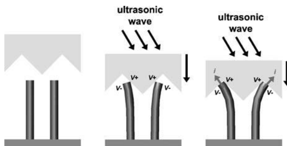
Fig. 9.17 Electrical power generation driven by ultrasonic waves. (a) The nanogenerator is based on an array of vertical ZnO nanowires. The top electrode has triangular trenches and is covered by a thin Pt film. (b) An ultrasonic wave drives the top electrode down, bending the ZnO nanowires and creating opposite piezoelectric potentials on the stretched and compressed sides of the nanowires. (c) The top electrode is driven further down, to the point where the compressed side of the nanowires is also in contact with the top electrode, resulting in a piezoelectric discharge and electrical current flow. (From [104]. Reproduced with permission from AAAS)
