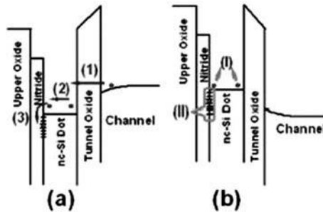
Fig. 8.9 (a) Writing and (b) erasure processes in nitrated nc-Si dot-based memory devices. (1) Direct tunneling from channel to nc-Si dot; (2) trapping on QC levels; (3) trapping at nc-Si/SiN x interface; (I) QC levels; (II) interface traps [5]. Reused with permission from Shaoyun Huang and Shunri Oda, Applied Physics Letters , 87 , 173107, 2005. Copyright © 2005, American Institute of Physics
