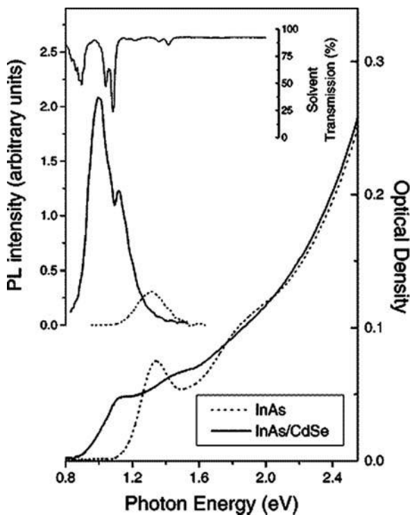
Fig. 8.20 InAs and InAs/CdSe nanocrystals absorption (optical density) and PL spectra [43]. Insert: toluene transmission spectrum.
