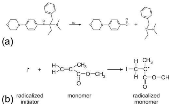
Fig. 12.3 (a) Cleavage of a photoinitiator, 2-benzyl-2-dimethylamino-4'-morpholinobutyrophenone, results from UV photon absorption; (b) radical polymerization of methyl methacrylate (MMA): I • is an initial radical or an intermediate in the reaction chain
