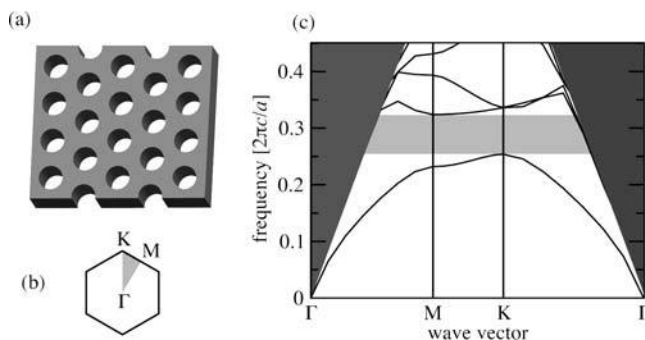
Fig. 11.6 (a) Photonic crystal slab. (b) Brillouin zone, with irreducible Brillouin zone shown in gray. (c) Band structure for TE-like modes, with light cone shown in dark gray and photonic band gap shown in light gray
