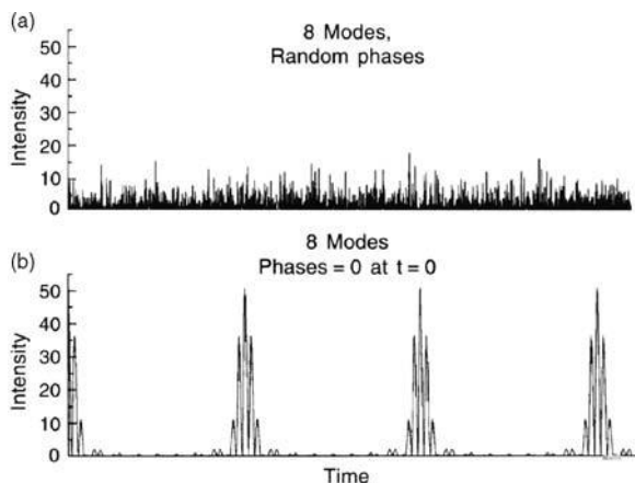
Fig. 12.6 Laser output simulation for eight modes: (a) random phase—continuous wave (CW) operation; (b) mode-locked operation
