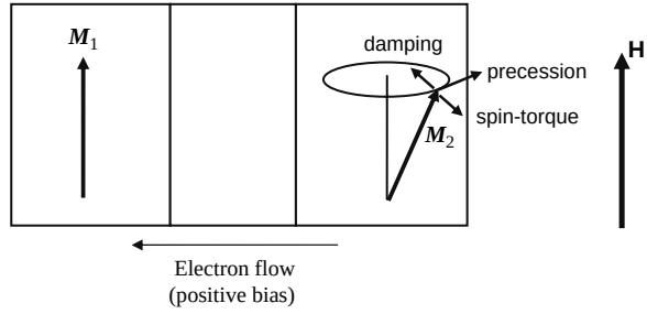
Fig. 5.15 Steady-state magnetization precession is achieved when the spin torque cancels the damping
