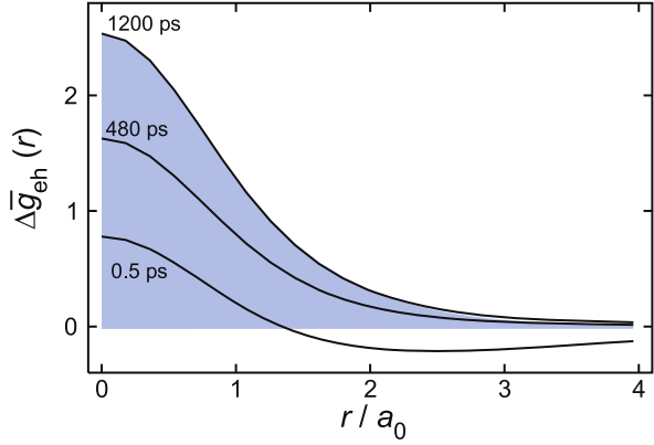
Fig. 10.10 Pair correlation function \Delta g_{eh}(r) for the lattice temperature of T = 10 K and carrier density n = 2 \times 10^4 \text{ cm}^{-1} at different times. The absolute square of the 1s-exciton wavefunction is shown as shaded area . (From Hoyer et al. [21])
