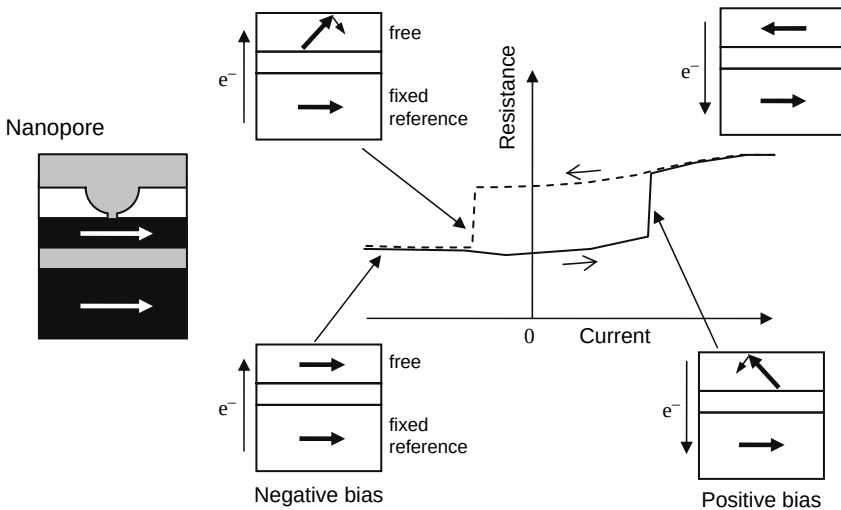
Fig. 5.12 Magnetization reversal by spin torque
