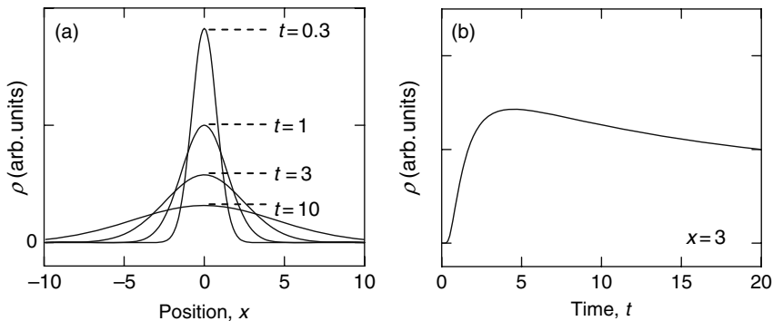
Fig. 5.34 (a) Solution to the diffusion equation at different times. The diffusion constant D is set to 1 for clarity. (b) The distribution of transit times of a particle starting at the origin and arriving at x = 3
