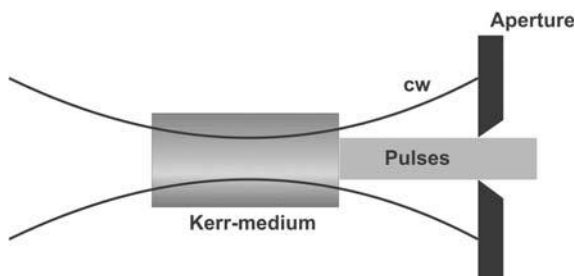
Fig. 12.7 The principle of Kerr lens mode-locking
