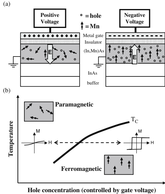
Fig. 5.23 Electric field control of carrier-mediated ferromagnetism
