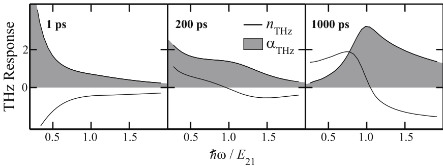
Fig. 10.11 Computed THz absorption ( shaded area ) and refractive index changes ( solid line ) for different THz probe delays after non-resonant excitation. Here, E_{2p-1s} = 5 is the energy difference between 1s and 2p states. (From Kira and Koch [97])
