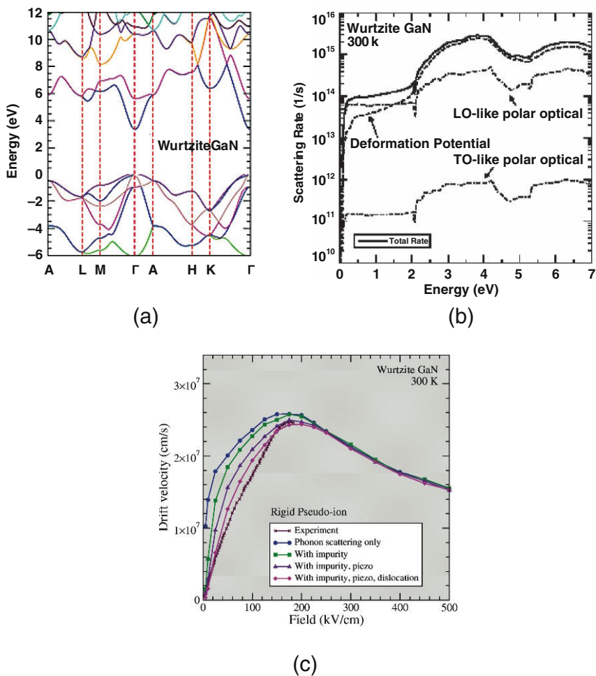
Fig. 6.8 Calculated bandstructure (a), rigid-ion scattering rates (b), and calculated velocity-field characteristics (c) from the CMC simulator for Wurtzite GaN at 300 K. Reprinted with permission from Ref. [39], Copyright 2004, Institute of Physics Publishing
