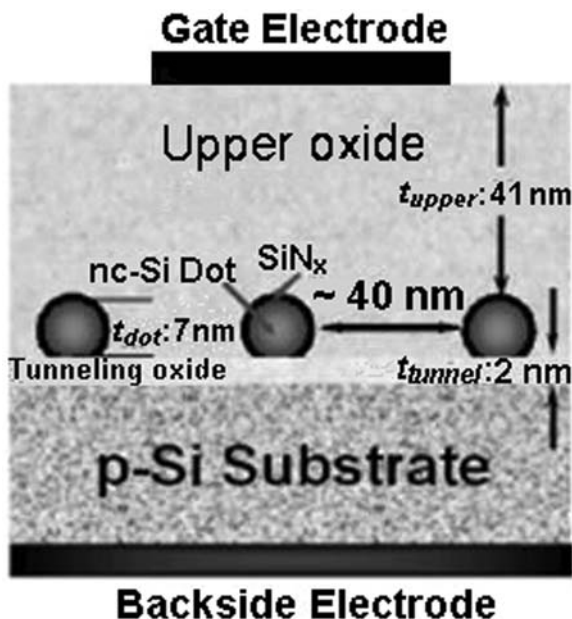
Fig. 8.7 The structure of the nitrided nc-Si dot memory [5]. Reused with permission from Shaoyun Huang and Shunri Oda, Applied Physics Letters, 87 , 173107, 2005. Copyright © 2005, American Institute of Physics
