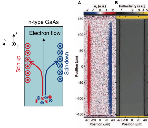
Fig. 5.35 ( Left ) General behavior of the spin Hall effect, where an unpolarized charge current generates a transverse spin current. ( Right ) Magneto-optical imaging of the spin Hall effect in n-type GaAs, from Ref. [159]. Reprinted with permission from AAAS
