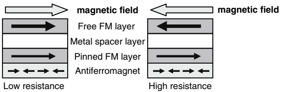
Fig. 5.18 GMR spin valve as a magnetic field sensor
