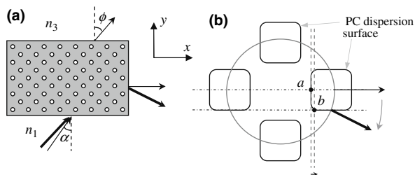
Fig. 11.30 A phase prism. (a) Device schematic; (b) dispersion surface
